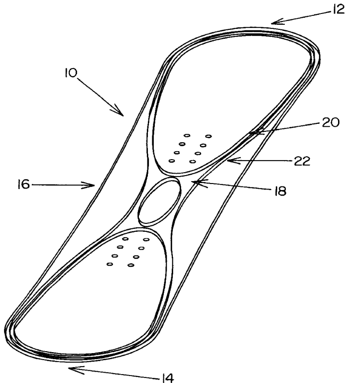
STRUCTURAL COMPONENTS MIRRORED ABOUT THE NEUTRAL AXIS OF THE SNOWBOARD.
