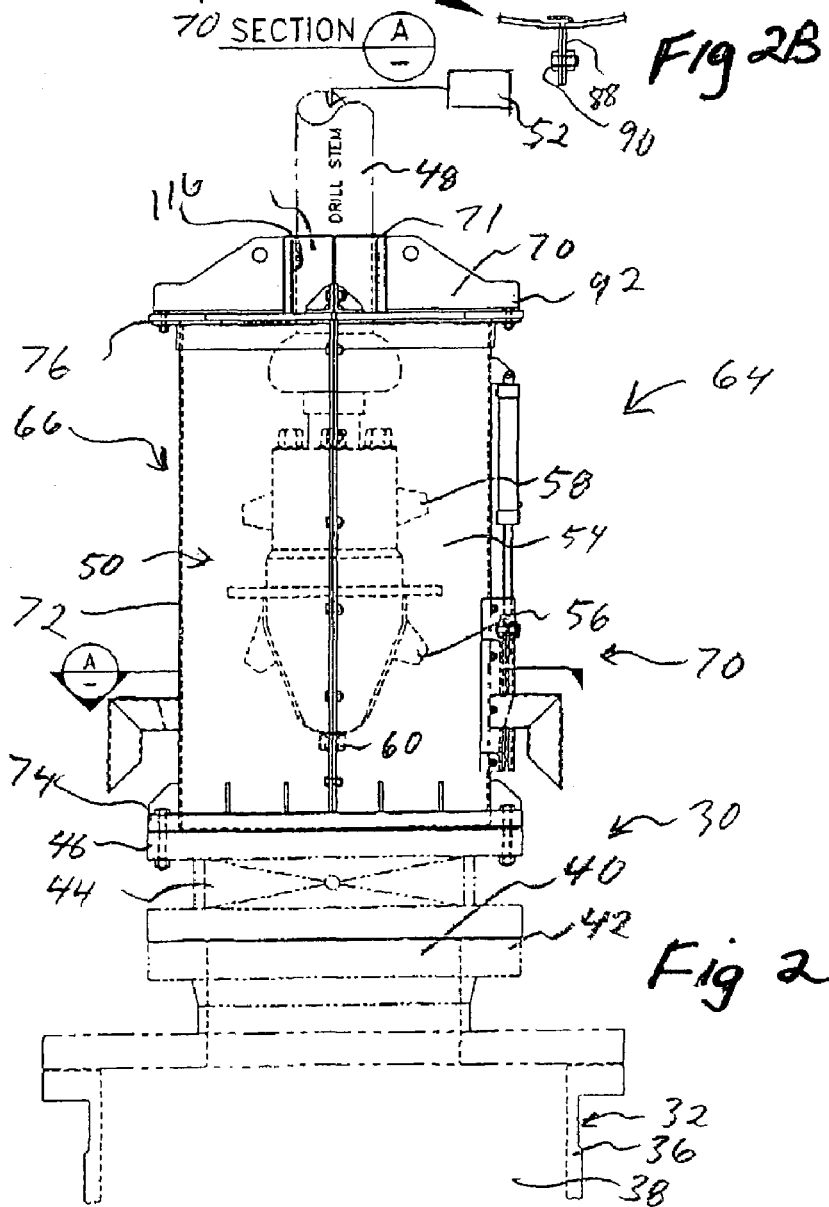
DRILL STEM RETRACTED (SIDE)
